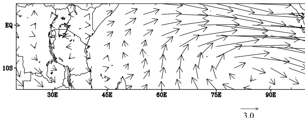
Figure8: (a) The composite wind flow pattern at 850 hPa during (a) positive IOD (b) negative IOD of 1981 to 2010 climatology.
