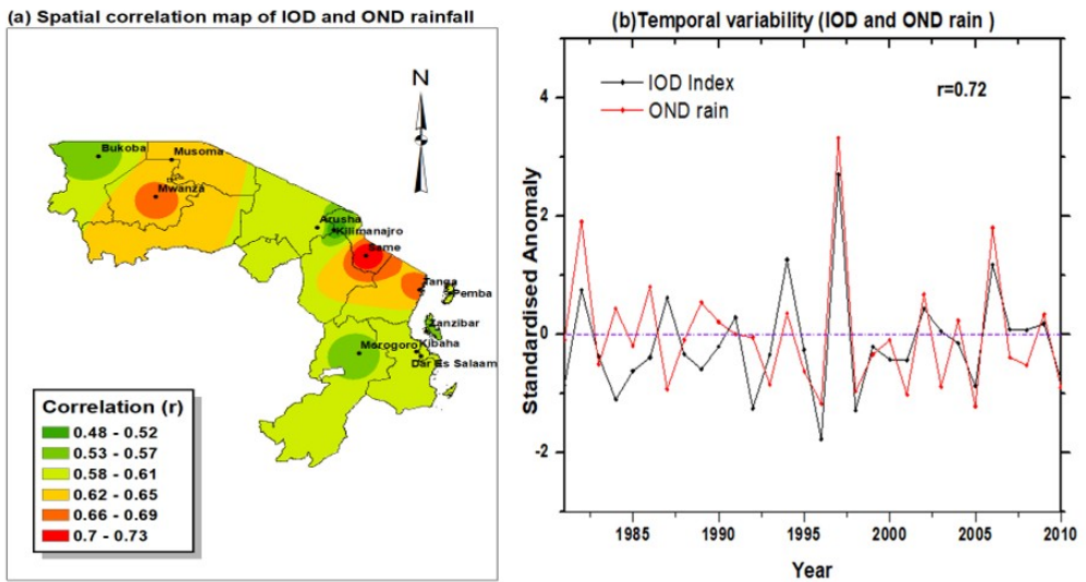
Figure6: (a) The spatial pattern of the correlation coefficient (b) temporal variability of the mean IOD indices during October to December and the OND rains over the bimodal rainfall regime of Tanzania based on 1981 to 2010 climatology.
