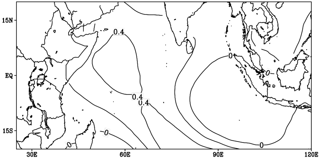
(a) Composite sea surface temperature (+ve IOD)
