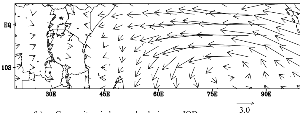
(b) Composite wind anomaly, during -ve IOD
